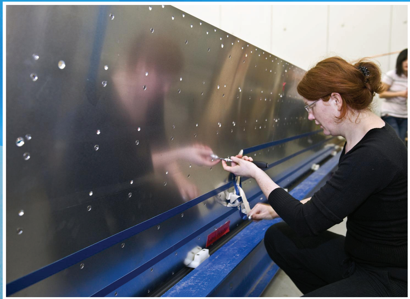
◀ Installing the station 5 tracking chamber in the test beam area (ALICE)
